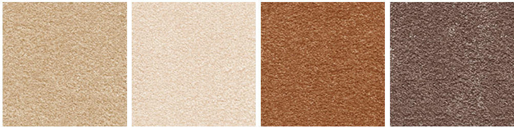
SIRIUS 30
